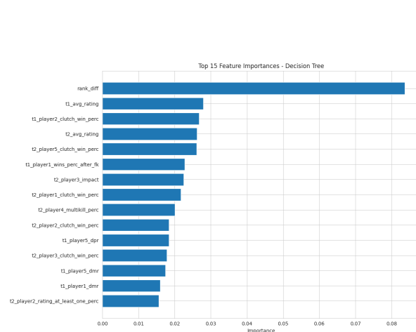
Figure 12: Top fifteen features: Decision Tree importance.
